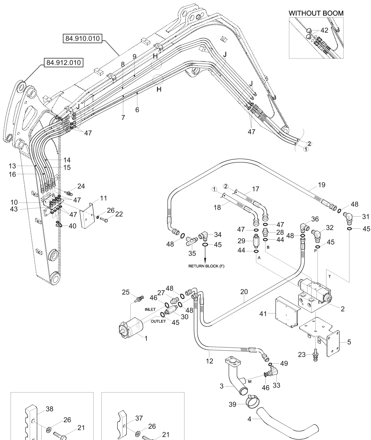
DETAIL J
